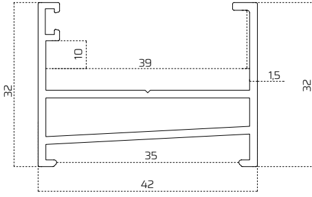
Alt Baza Profili / Lower Base Profile
