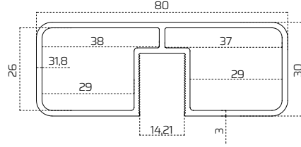
K peŐte Profili / Gunwale Profile
