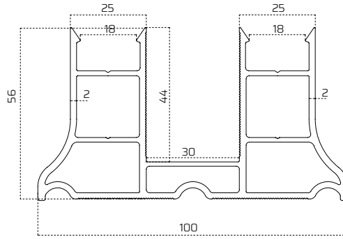
Baza Profili / Base Profile
