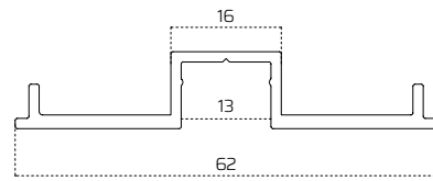
Dikme Kapak Profili / Sewing Cover Profile
