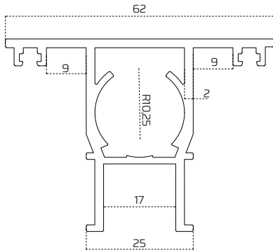
Alt Baza Profili / Lower Base Profile
