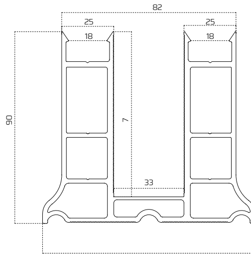
B y k Baza Profili / Big Base Profile
